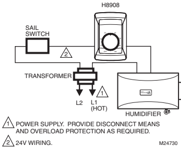
Fig. 15. Wiring H8908 in line with sail switch and humidifier.
