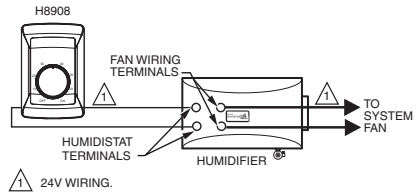
⚠ 24V WIRING. NOTE: FOLLOW THE INSTALLATION INSTRUCTIONS INCLUDED WITH THE STEAM HUMIDIFIER TO WIRE THE SYSTEM FAN. M24731
