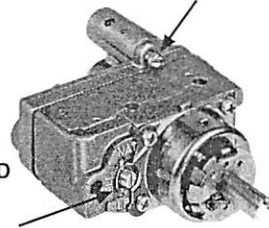
PHOTO 1 MODEL UAF TOP BURNER PILOT ADJUSTMENT
