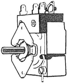
TYPES "B", "E" & "F" HAS 3 AUXILIARY SWITCH TERMINALS
