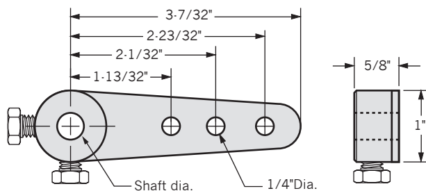
3 Hole Crank Arm
